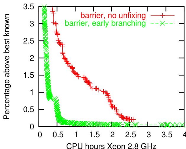
Figure 2: Different integrality strategies
